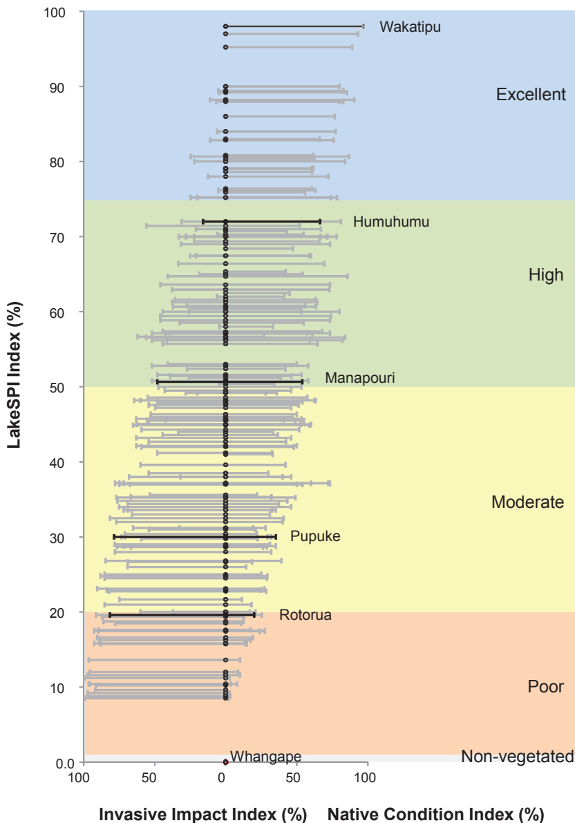
FIGURE 7 LakeSPI status for 236 lakes based on the most recent survey data. LakeSPI Index is plotted on the vertical axis (black circles), with the Native Condition Index plotted as a horizontal grey line on the right, and Invasive Impact Index on the left. Position of six benchmark lakes is indicated. A LakeSPI score of 0% represents the widespread loss of submerged plants from a lake (i.e., a non-vegetated state), which is recognised as more impaired than a lake dominated by an invasive macrophyte.
