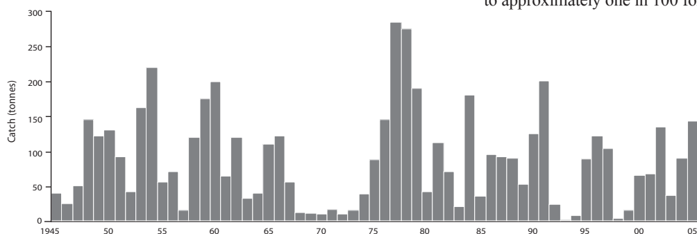
FIGURE 4 Commercial flounder catches from Lake Ellesmere/Te Waihora between 1945 and 2005 (Source: Jellyman and Smith 2009).
