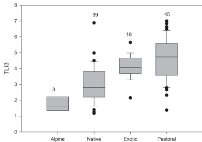
FIGURE 5 Box and whisker plots showing differences in Trophic Level Index (TLI3: based on chlorophyll a, total nitrogen and total phosphorus) in four classes of predominant catchment land cover. Numbers indicate sample size. Horizontal lines within boxes show median values, boxes show 25–75% data ranges, whiskers show 5–95% ranges, and circles outliers outside the 5–95% ranges (Source: Verburg et al. 2010).
