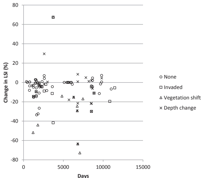
FIGURE 6 The direction and magnitude of change in LakeSPI score (LSI %) with time (days) between lake surveys, where the nature of change is identified as: Depth change (vegetation maximum depth changed by an average of \geq 2 m; 24 lakes); invaded (recorded the presence of a more invasive weed; 15 lakes); vegetation shift (switch between vegetated and non-vegetated status at the majority of lake sites; 10 lakes); none (no obvious cause of change; 48 lakes).
