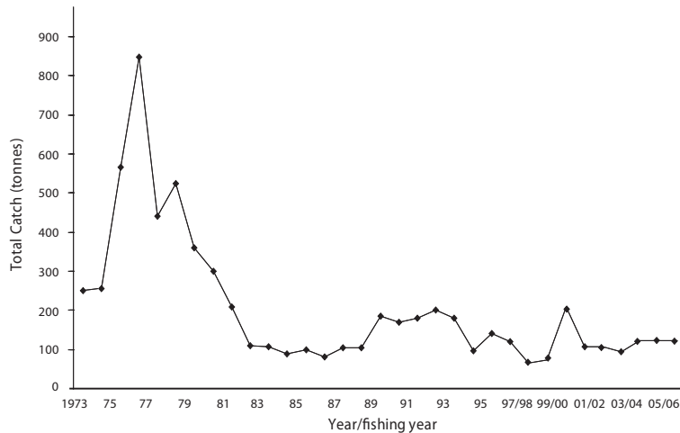
FIGURE 3 Trends in commercial eel catches from Lake Ellesmere/Te Waihora between 1973 and 2006 (Source: Jellyman and Smith 2009).
