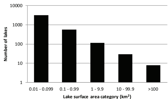
FIGURE 1 Total number of lakes in New Zealand per surface area category. (Data source: Leathwick et al. 2010).
